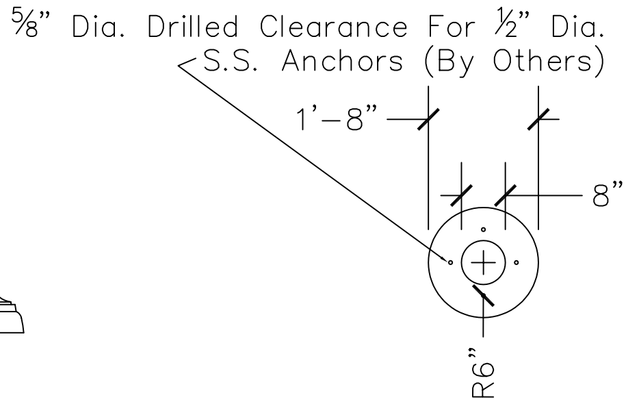
Base Anchorage
